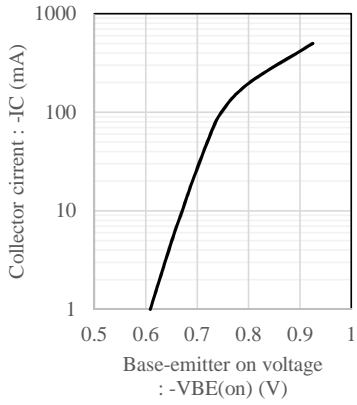
Fig.1 VBE(on) - IC at VCE= -1V, Ta= 25C
