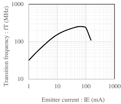
Fig.5 fT - IE at VCE= -1V, Ta= 25C
