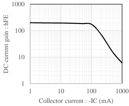
Fig.2 hFE - IC at VCE= -1V, Ta= 25C
