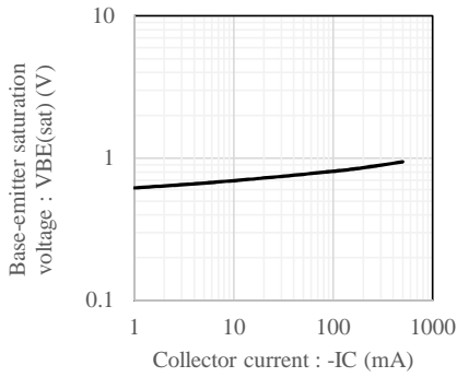
Fig.4 VBE(sat) - IC at IC/IB= 10, Ta= 25C
