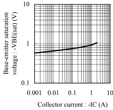
Fig.5 VBE(sat) - IC at IC/IB= 20, Ta= 25C
