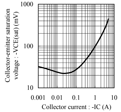
Fig.3 VCE(sat) - IC at IC/IB = 5, Ta = 25C
