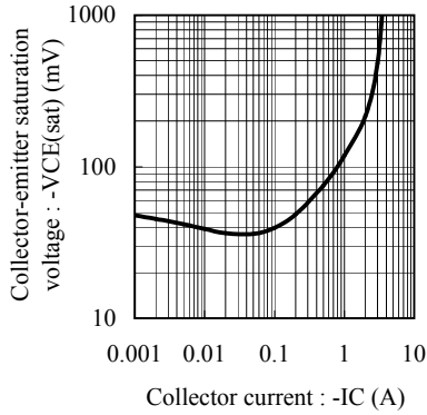
Fig.4 VCE(sat) - IC at IC/IB = 10, Ta = 25C
