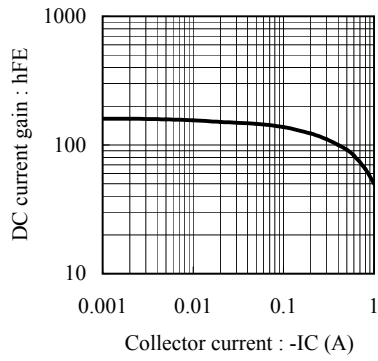
Fig.1 hFE - IC at VCE= -1V, Ta= 25C
