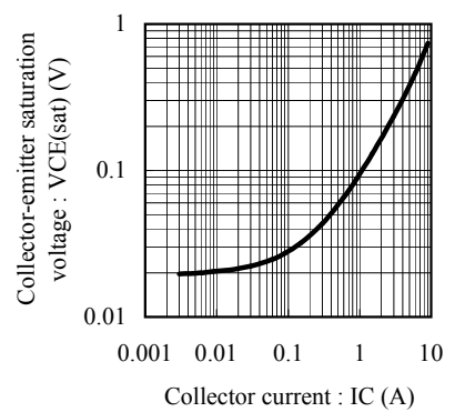
Fig.6 VCE(sat) - IC at IC/IB= 150, Ta= 25C
