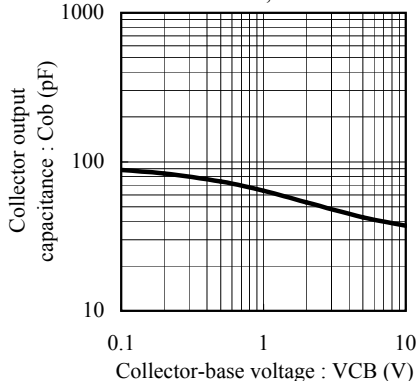
Fig.10 Cob - VCB at f= 1MHz, Ta= 25C
