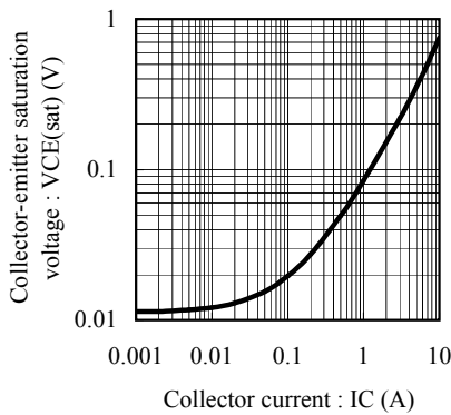
Fig.7 VCE(sat) - IC at IC/IB= 200, Ta= 25C
