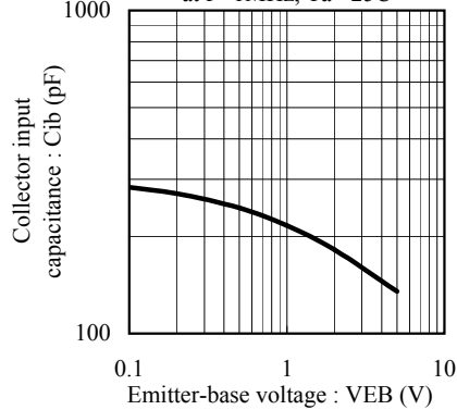
Fig.11 Cib - VEB at f= 1MHz, Ta= 25C
