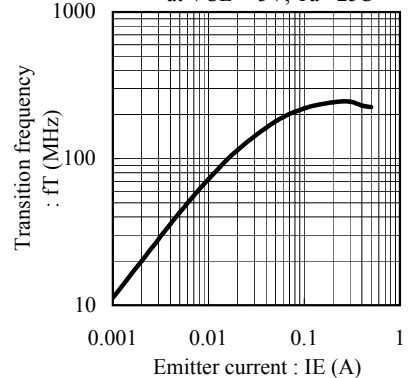
Fig.9 fT - IE at VCE= -5V, Ta= 25C
