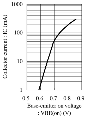
Fig.1 VBE(on) - IC at VCE= 10V, Ta= 25C
