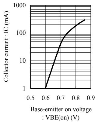
Fig.1 IC - VBE(on) at VCE=10V, Ta= 25C
