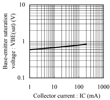
Fig.4 VBE(sat) - IC at IC/IB= 10, Ta= 25C
