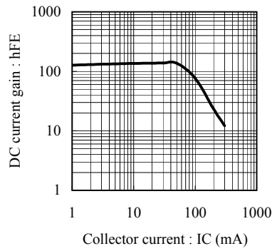
Fig.2 hFE - IC at VCE= 10V, Ta= 25C
