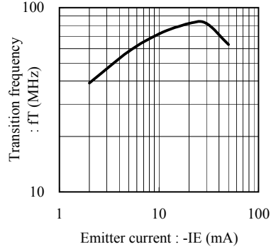
Fig.5 fT - IE at VCE= 10V, Ta= 25C
