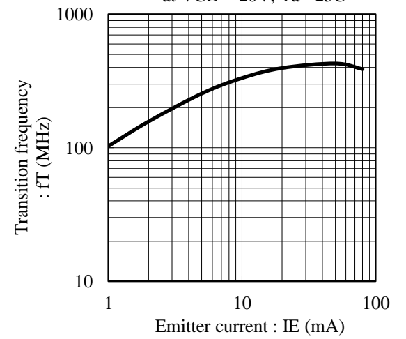
Fig.6 fT - IE at VCE= -20V, Ta= 25C
