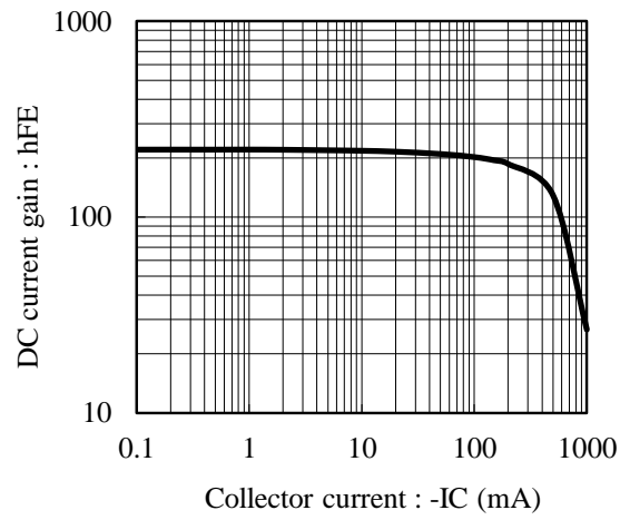
Fig.2 hFE - IC at VCE= -10V, Ta= 25C
