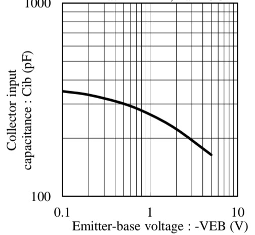
Fig.9 C_{ib} - V_{EB} at f = 1MHz, T_a = 25^\circ C
