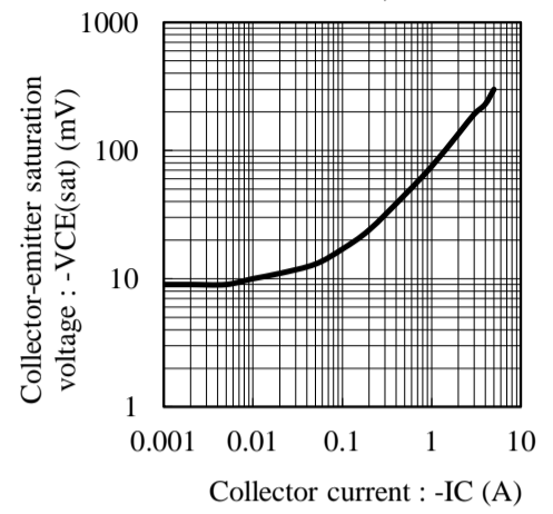
Fig.3 V_{CE(sat)} - I_C at I_C/I_B = 10, T_a = 25^\circ C
