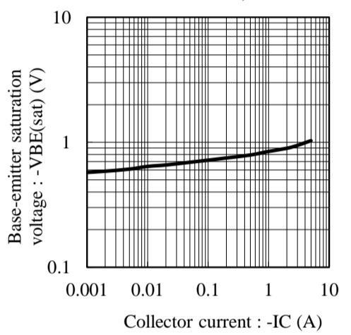
Fig.6 V_{BE(sat)} - I_C at I_C/I_B = 20, T_a = 25^\circ C
