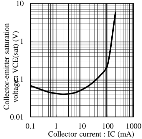
Fig.4 VCE(sat) - IC at IC/IB= 10, Ta= 25C
