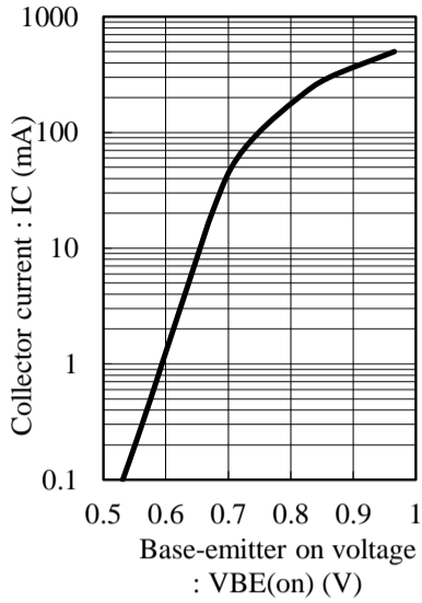
Fig.1 IC - VBE(on) at VCE= 10V, Ta= 25C
