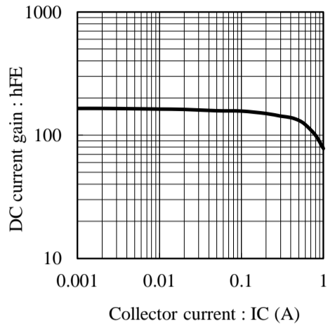
Fig.1 hFE - IC at VCE= 1V, Ta= 25C
