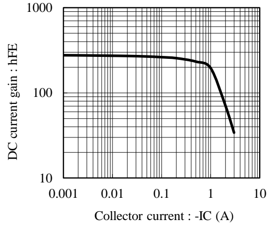
Fig.2 hFE - IC at VCE= -2V, Ta= 25C
