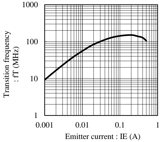
Fig.5 fT - IE at VCE= -5V, Ta= 25C
