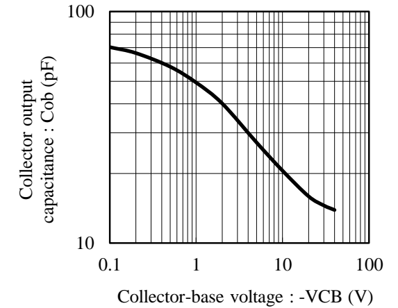
Fig.6 Cob - VCB at f= 1MHz, Ta= 25C
