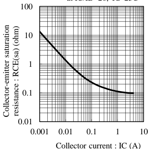
Fig.X RCE(sat) - IC at IC/IB=20, Ta=25C
