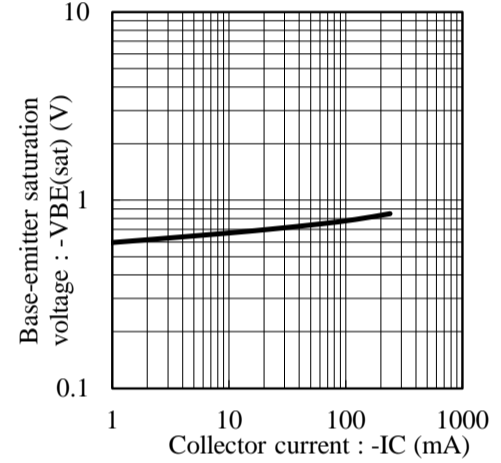
Fig.6 VBE(sat) - IC at IC/IB = 24, Ta = 25C
