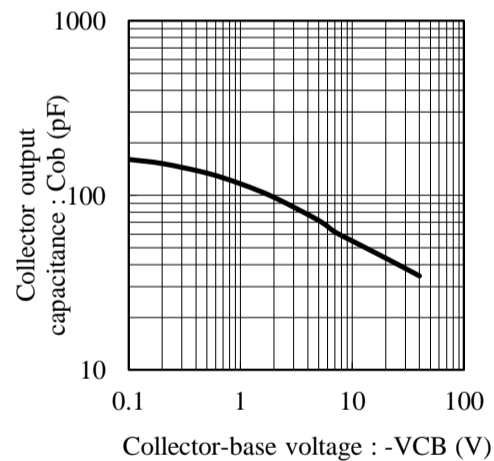
Fig.7 Cob - VCB at f= 1MHz, Ta= 25C
