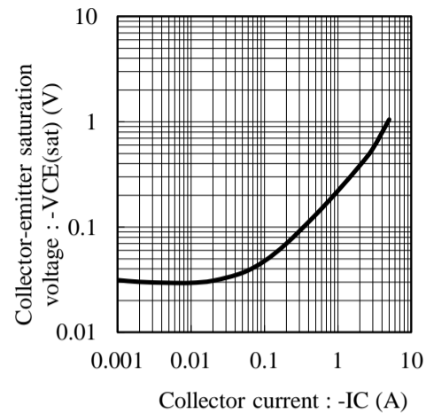
Fig.3 VCE(sat) - IC at IC/IB= 8, Ta= 25C
