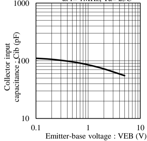
Fig.8 Cib - VEB at f= 1MHz, Ta= 25C
