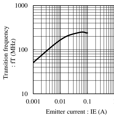
Fig.5 fT - IE at VCE= -10V, Ta= 25C
