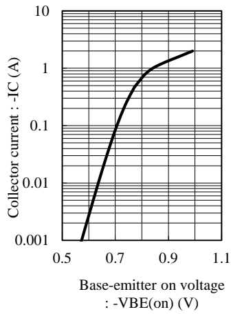
Fig.1 IC - VBE(on) at VCE= -5V, Ta= 25C
