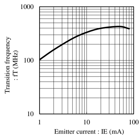
Fig.6 fT - IE at VCE = -20V, Ta = 25C
