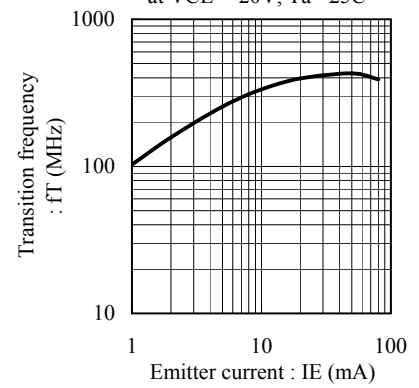
Fig.6 fT - IE at VCE= -20V, Ta= 25C
