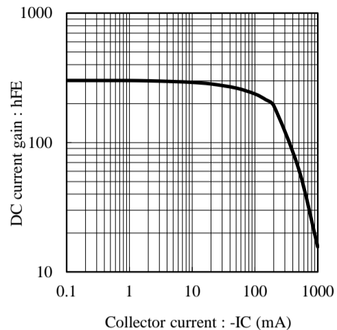
Fig.3 hFE - IC at VCE = -2V, Ta = 25C
