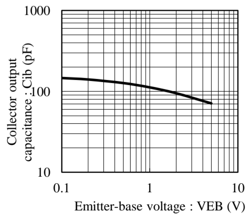
Fig.10 C_{ib} - V_{EB} at f = 1MHz, T_a = 25C
