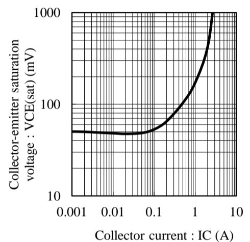
Fig.6 V_{CE(sat)} - I_C at I_C/I_B = 100, T_a = 25C
