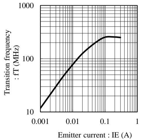
Fig.6 fT - IE at VCE= -2V, Ta= 25C
