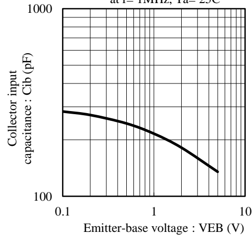
Fig.11 Cib - VEB at f= 1MHz, Ta= 25C
