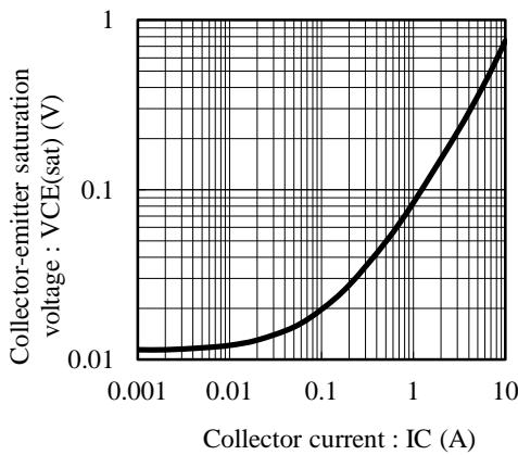
Fig.7 VCE(sat) - IC at IC/IB= 200, Ta= 25C
