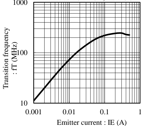
Fig.9 fT - IE at VCE= -5V, Ta= 25C
