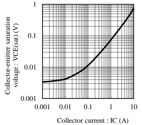
Fig.3 VCE(sat) - IC at IC/IB= 20, Ta= 25C
