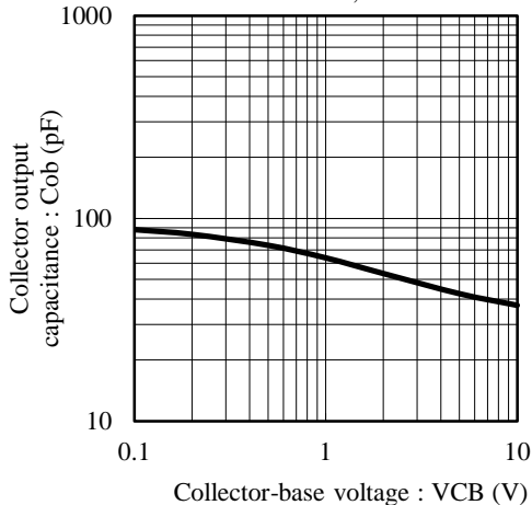
Fig.10 Cob - VCB at f= 1MHz, Ta= 25C
