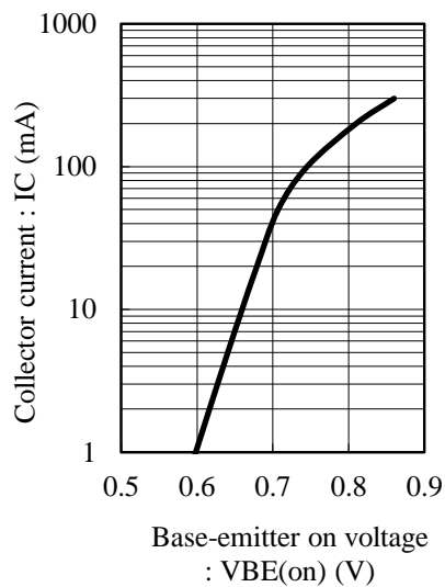
Fig.1 IC - VBE(on) at VCE=10V, Ta= 25C
